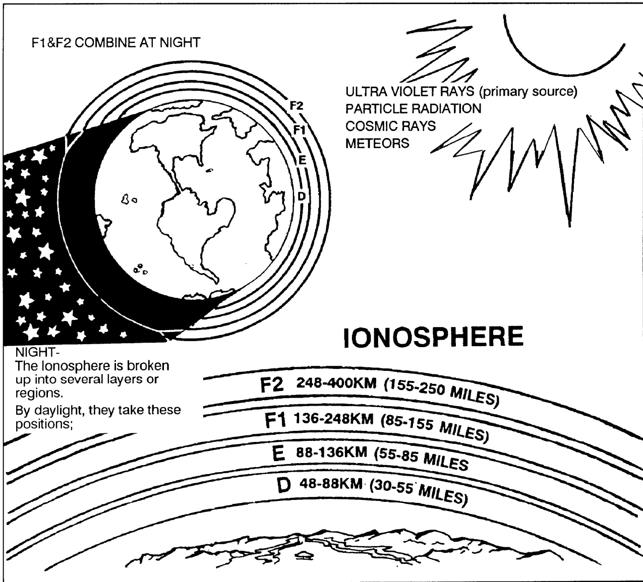
Figure D-3. Structure of the ionosphere.
